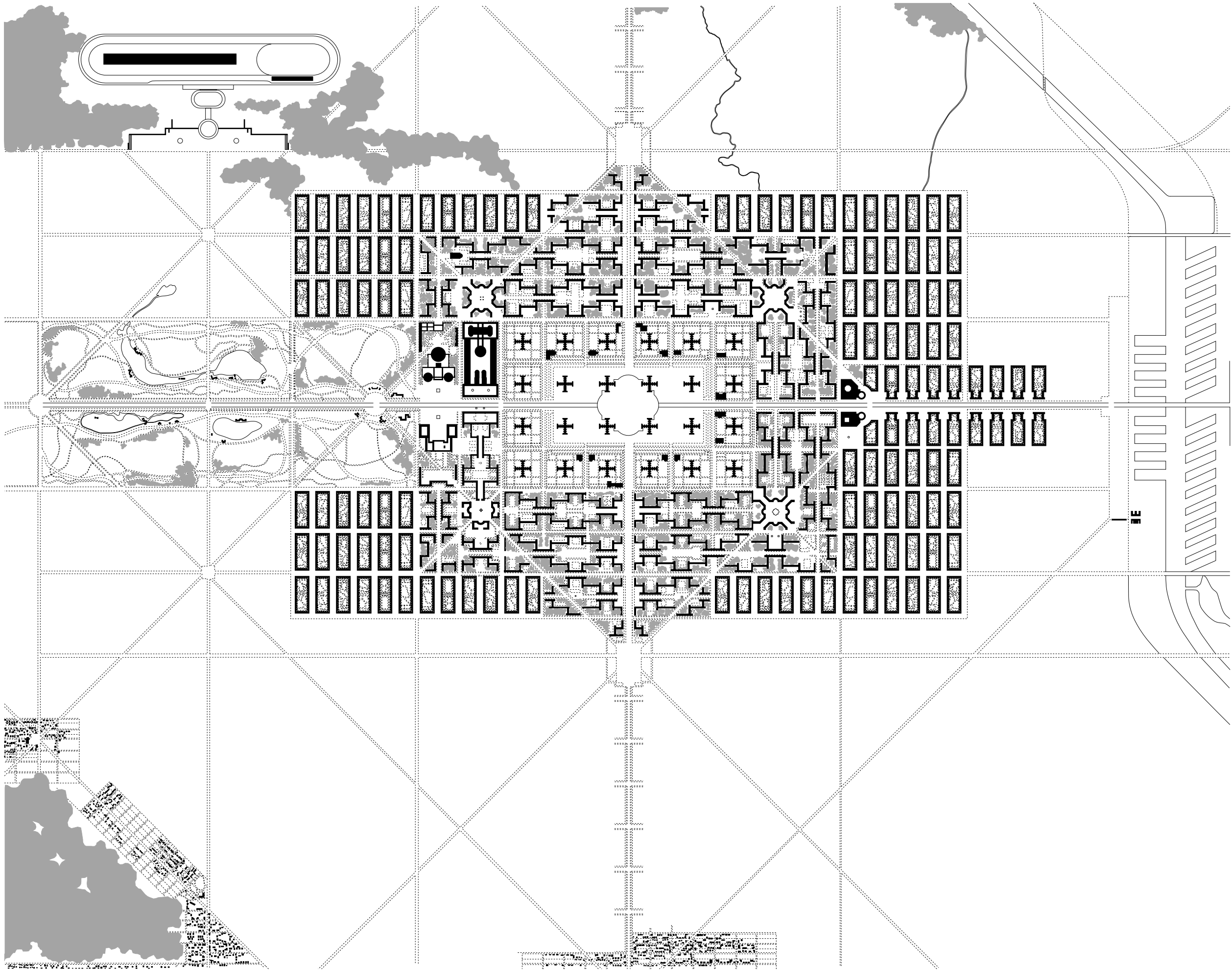
CITY FOR THREE MILLION, BY LE CORBUSIER, CA 1924
